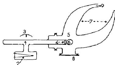
Fig. 1. Experimental apparatus: 1, lamp; 2, titanium wires; 3, microwave power antenna; 4, LiF window; 5, photolysis cell; 6, gas input and pressure measurements; 7, Wood's horns; 8, quartz observation window; 9, gas output and vacuum.
