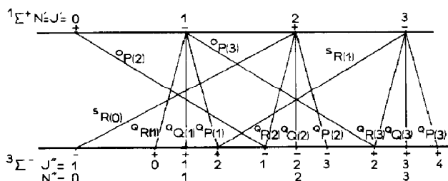
Fig. 12. Schematic diagram for the rotational levels of the NH(ND) b ^1\Sigma^+ \rightarrow X \ ^3\Sigma^- transition.
