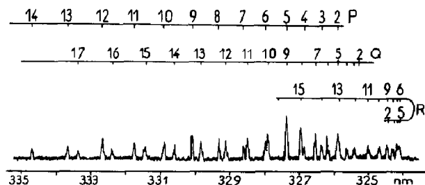
Fig. 4. Emission spectrum in the second order of the 0 - 0 NH c^1\pi \rightarrow a^1\Delta transition formed during the photolysis of ammonia by Kr resonance lamp.
