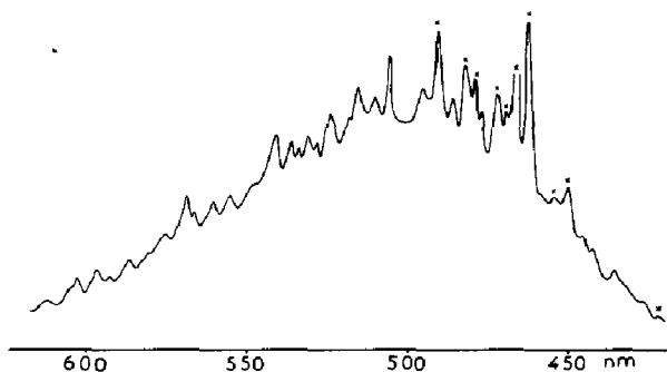
Fig. 2. Emission spectrum \text{NH}_2 \tilde{\text{A}}^2\text{A}_1 \rightarrow \tilde{\text{X}}^2\text{B}_1 transition formed during the photolysis of ammonia at 147 nm. * designates Xe scattered lines.
