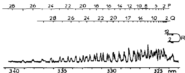
Fig. 5. Emission spectrum in the second order of the 0 - 0 ND c^1\pi \rightarrow a^1\Delta transition formed during the photolysis of ammonia- d_3 by Kr resonance lamp.
