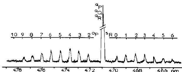
Fig. 11. Emission spectrum of ND b^1\Sigma^+ \rightarrow X^3\Sigma^- formed during the photolysis of ammonia- d_3 by Ar resonance lines.
