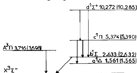
Fig. 13. Energy diagram of NH and ND. The energy values in eV, are the intervals between X^3\Sigma^- \nu = 0 level and excited states \nu = 0 levels. Values in parenthesis concern ND.
