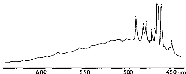
Fig. 3. Emission spectrum \text{ND}_2 \tilde{\text{A}}^2\text{A}_1 \rightarrow \tilde{\text{X}}^2\text{B}_1 transition formed during the photolysis of ammonia- d_3 at 147 nm. * designates Xe scattered lines.
