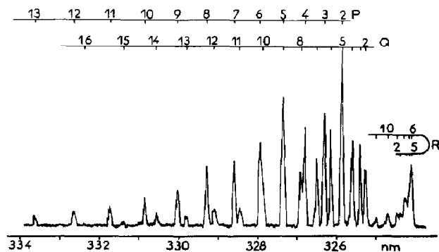
Fig. 6. Emission spectrum in the second order of the 0-0 \text{NH } c \ ^1\pi \rightarrow a \ ^1\Delta transition formed during the photolysis of ammonia- d_3 by Ar resonance lamp.
