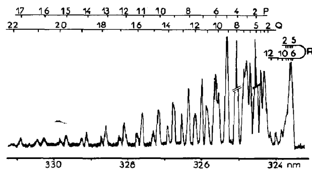
Fig. 7. Emission spectrum in the second order of the 0-0 \text{ND } c \ ^1\pi \rightarrow a \ ^1\Delta transition formed during the photolysis of ammonia- d_3 by Ar resonance lamp.
