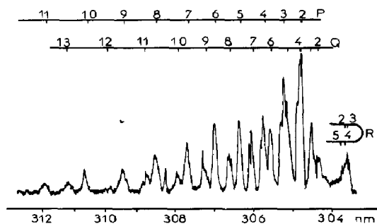
Fig. 8. Emission spectrum in the second order of the 1-0 \text{NH } c \ ^1\pi \rightarrow a \ ^1\Delta transition formed during the photolysis of ammonia- d_3 by Ar resonance lamp.
