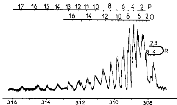
Fig. 9. Emission spectrum in the second order of the 1-0 ND c^1\pi \rightarrow a^1\Delta transition formed during the photolysis of ammonia- d_3 by Ar resonance lamp.
