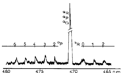
Fig. 10. Emission spectrum of NH b^1\Sigma^+ \rightarrow X^3\Sigma^- formed during the photolysis of ammonia- d_3 by Ar resonance lines.
